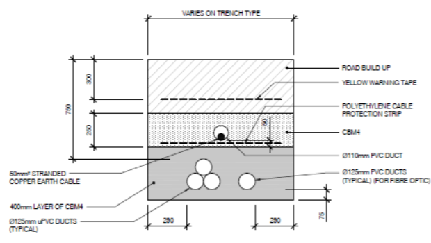
TYPICAL ROAD CROSSING DETAIL SCALE 1:20 [ 1 No. RADIAL ]
