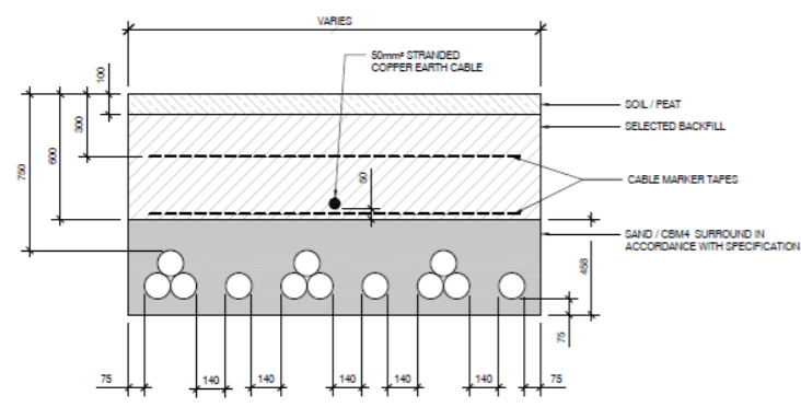
INDICATIVE CABLE TRENCH SCALE 1:20 [ 3 No. RADIALS ]
