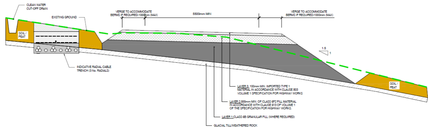
INDICATIVE NEW ACCESS TRACK SECTION SCALE 1:50
