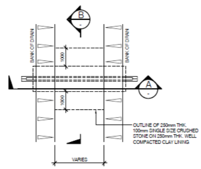
PLAN: TYPICAL TREFOIL FORMATION DRAIN CROSSING SCALE 1:100 [ 1 No. RADIAL ]
